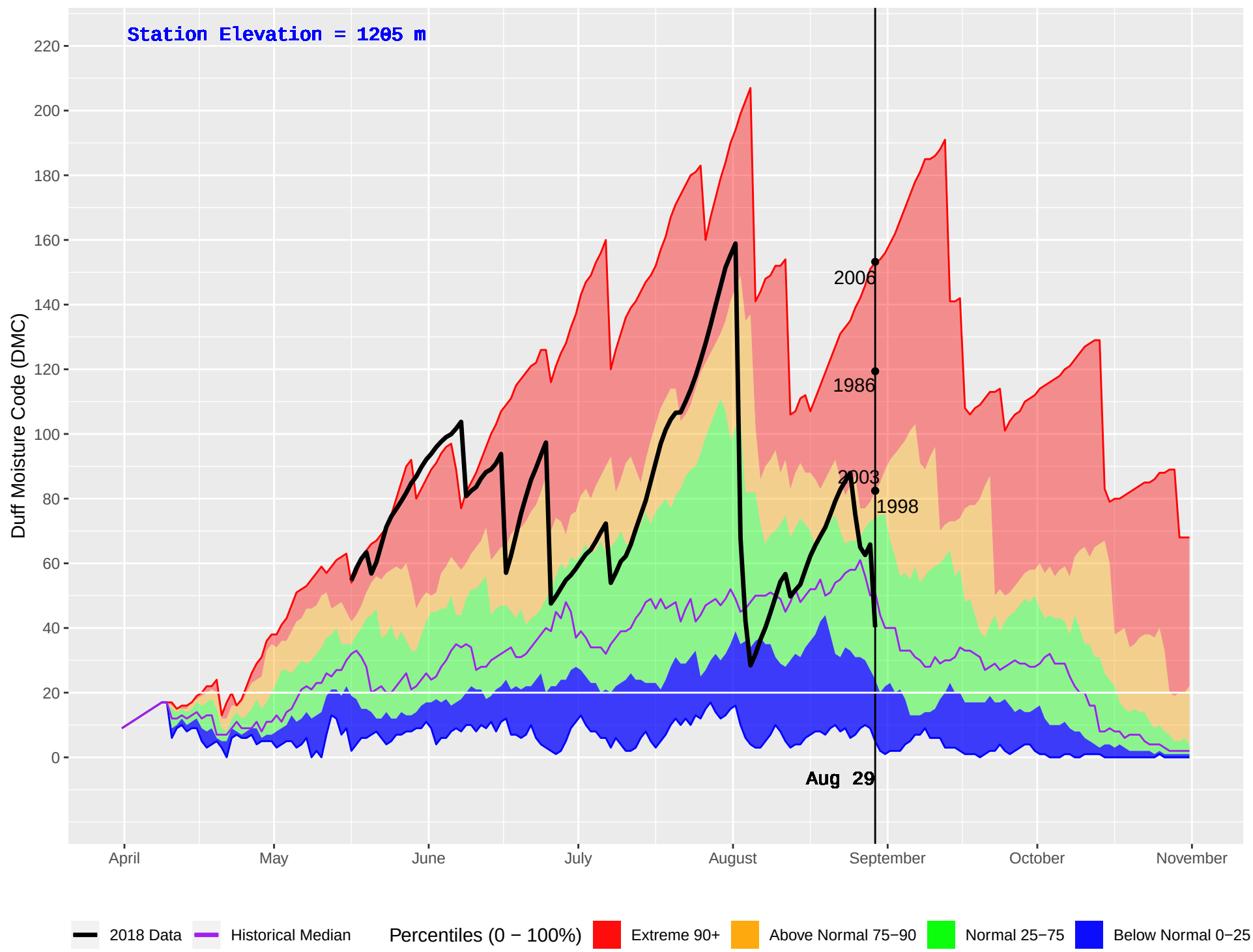
GWYNETH LAKE (309) : Historical (1986–2016) and Current (2018) Daily Duff Moisture Code (DMC)
