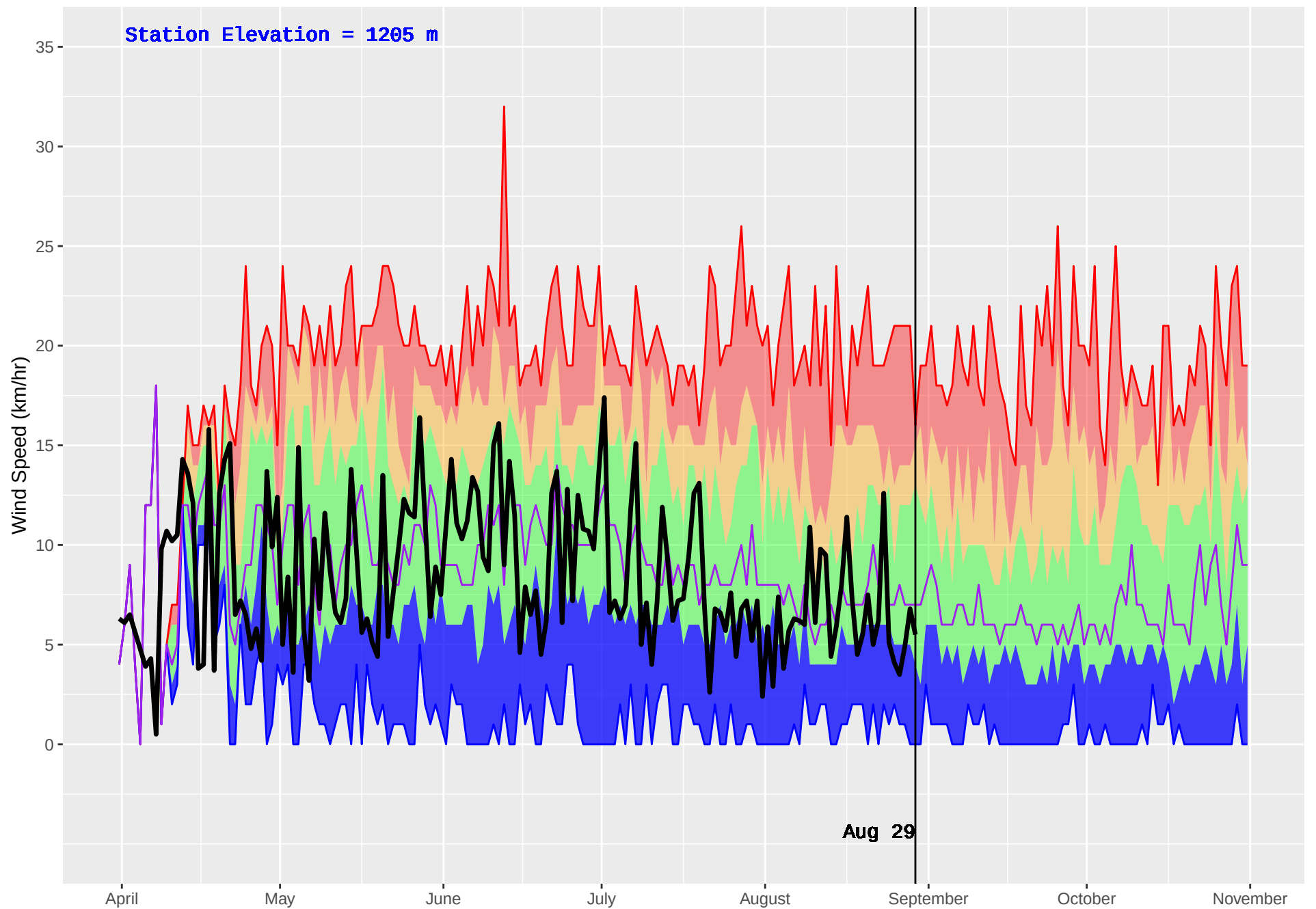
GWYNETH LAKE (309) : Historical (1986–2016) and Current (2018) Daily Wind Speed
