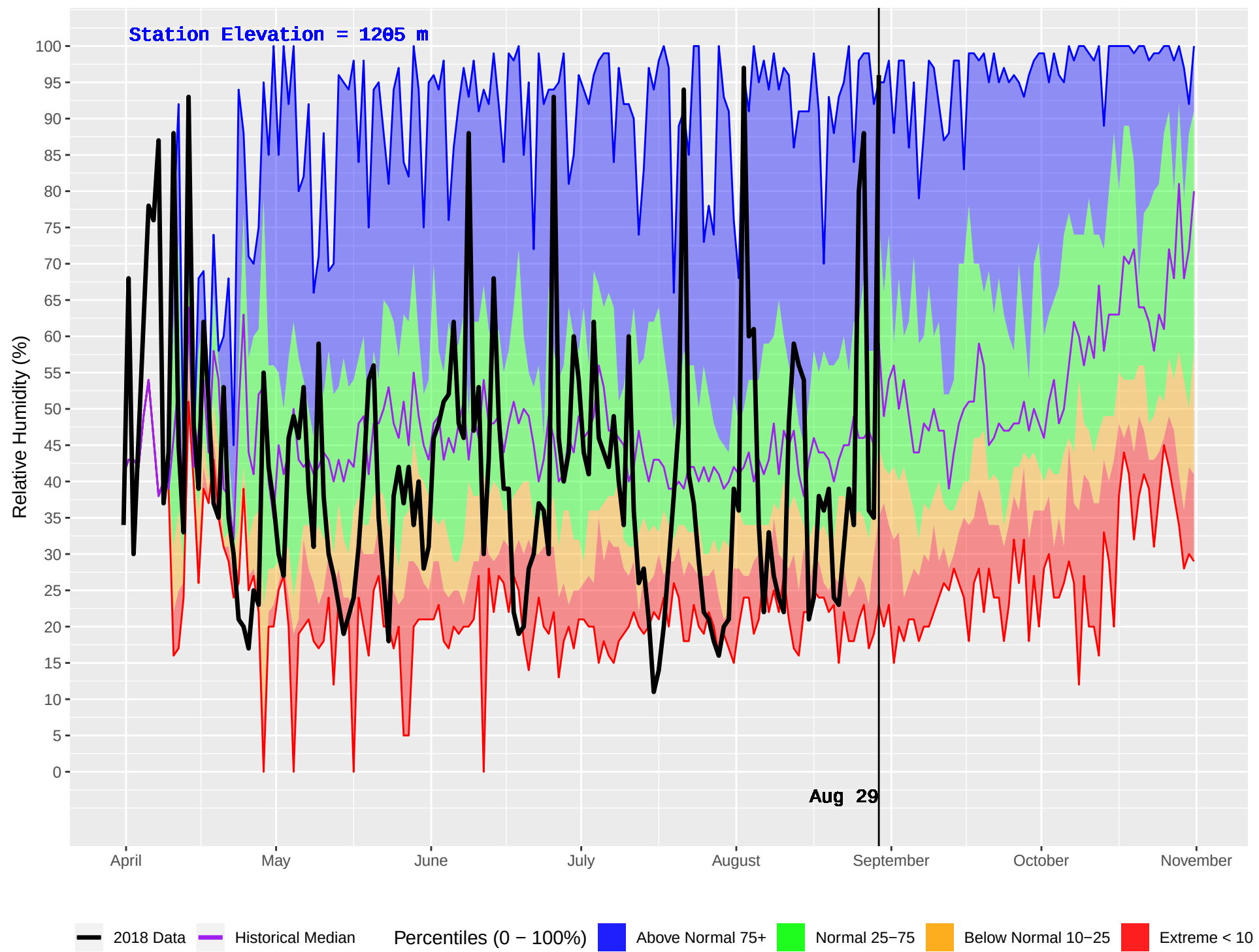
GWYNETH LAKE (309) : Historical (1986–2016) and Current (2018) Daily Relative Humidity
